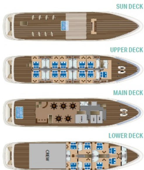
Main Deck
